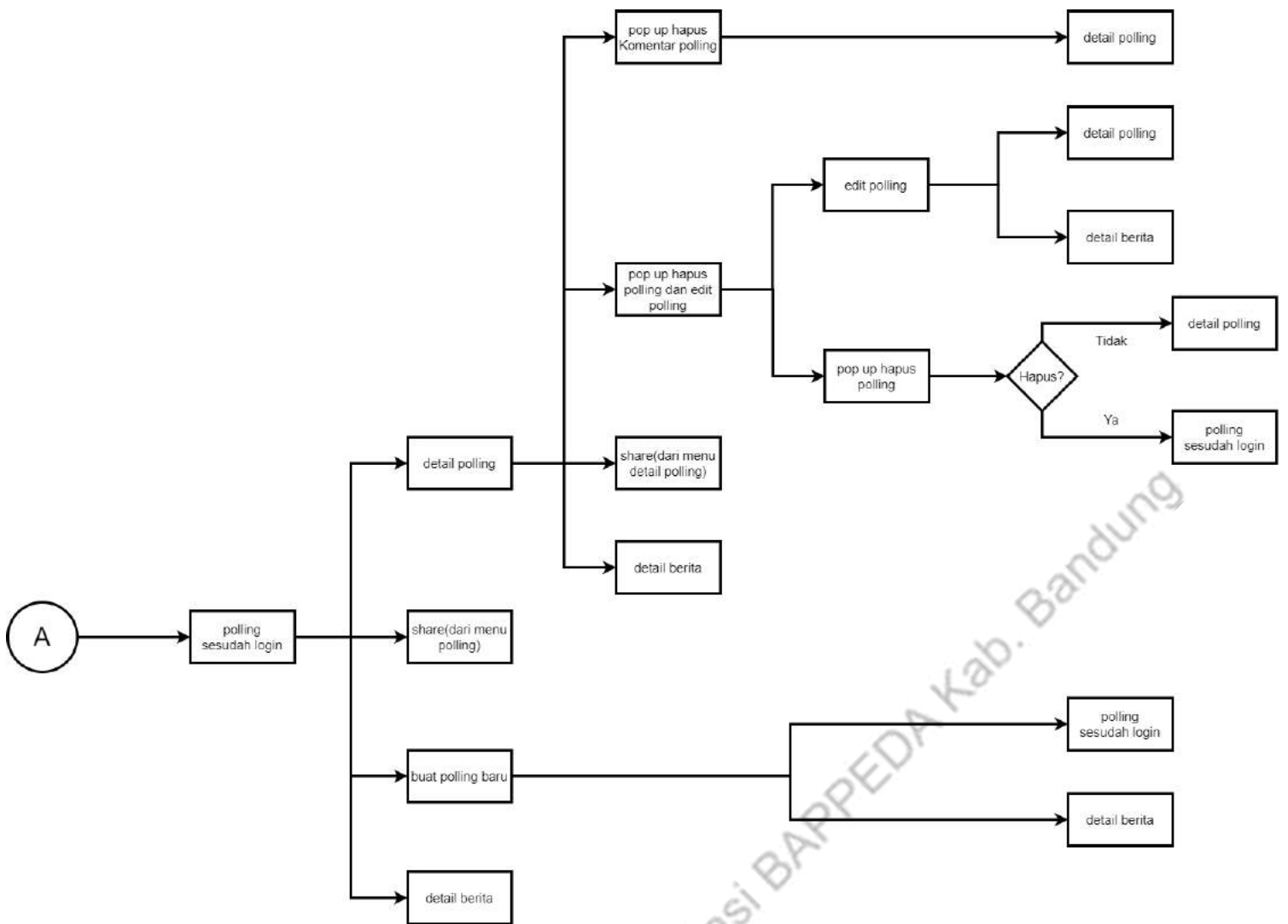
Gambar 10 UI Tree Polling (Admin)
