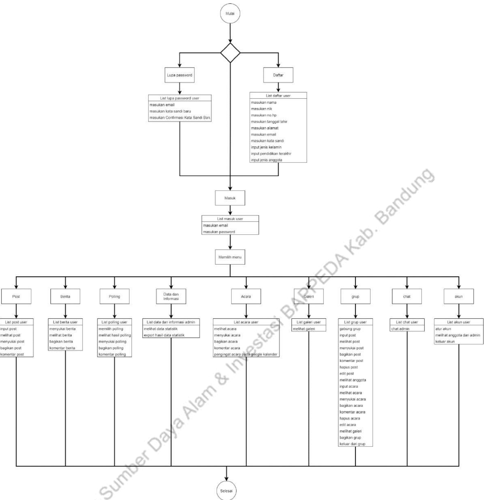
Gambar 5 Proses Bisnis User
