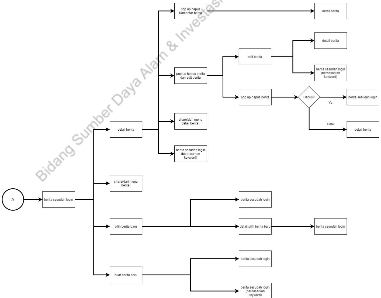
Gambar 9 UI Tree Berita (Admin)
