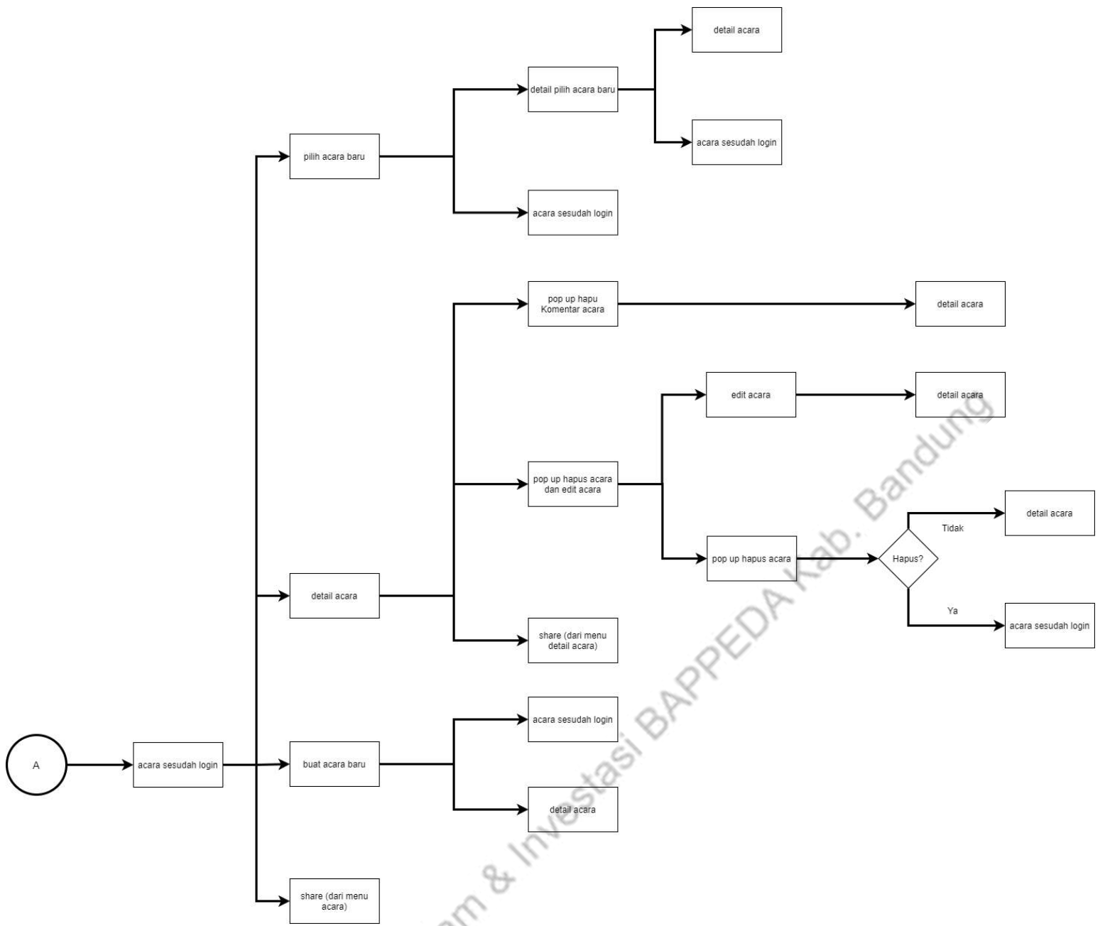
Gambar 13 UI Tree Acara (Admin)
