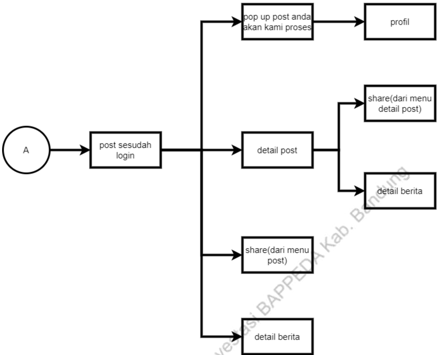
Gambar 19 UI Tree Posting (User)
