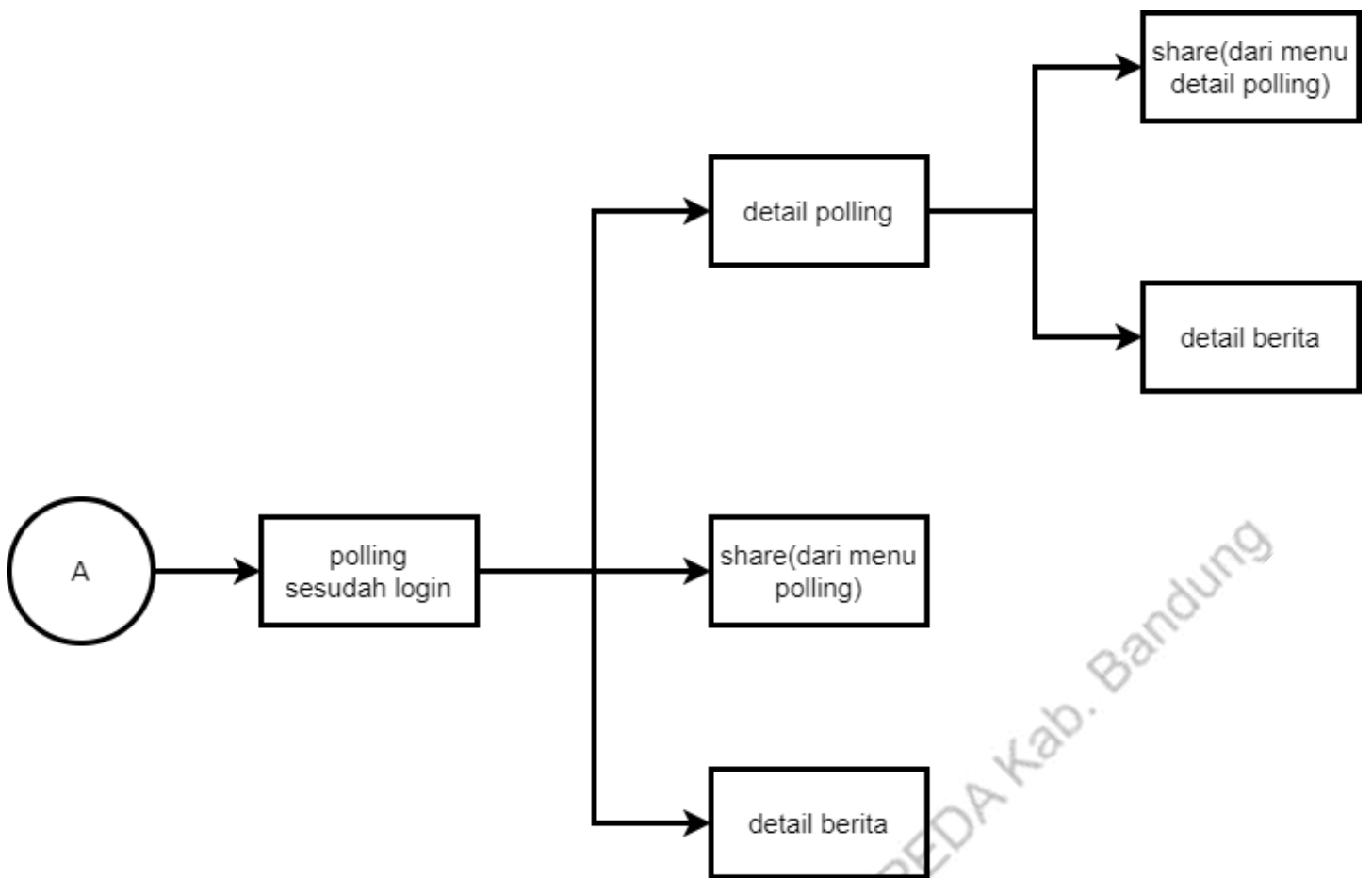
Gambar 21 UI Tree Polling (User)
